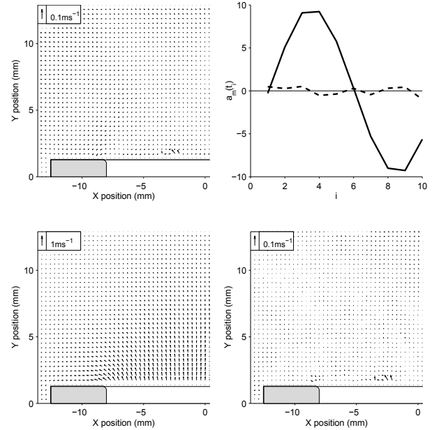
FIGURE 2 – Flow decomposition for r = 0.3 mm termination : p_{an} = 203 Pa. Top left : Streaming flow \tilde{\mathbf{u}}(x, y) . Top right : a_m(t_i) of first 2 POD modes ( - ) a_1 , ( - - - ) a_2 . Bottom left : \Phi_1(x, y) . Bottom right : \Phi_2(x, y) . Spatial maps show left half of termination, with grey areas representing termination wall.
