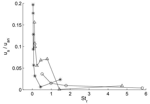
FIGURE 9 – Normalised jet velocity u_s against St_r . (*) r = 0.3 mm, ( \Delta ) r = 1 mm, ( \circ ) r = 4 mm.
