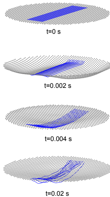
Figure 7: Snapshots of interaction of twelve snares with lower membrane, for a strike applied to the upper membrane, at times as indicated. The sample rate is 16 kHz, and the membrane is of parameters as described in the figures above. The wave speed in the snares is set to 30 m/s.
