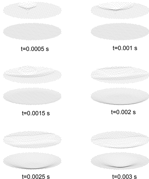
Figure 3: Snapshots of the time evolution of a coupled membrane system, at times as indicated. The upper and lower membranes have wave speeds of 95.2 m/s and 75.9 m/s, respectively, and are of radius 0.15 m. The cavity between them is of depth 0.3 m. The scheme described in Section 3 is used, at a sample rate of 16 kHz.
