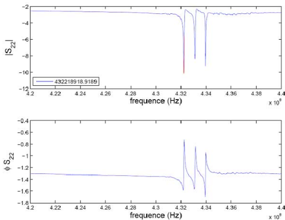
Figure 9: Electrical results
