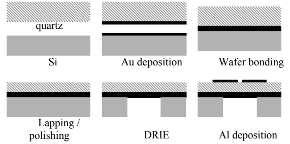
Figure 3: Process Flow
