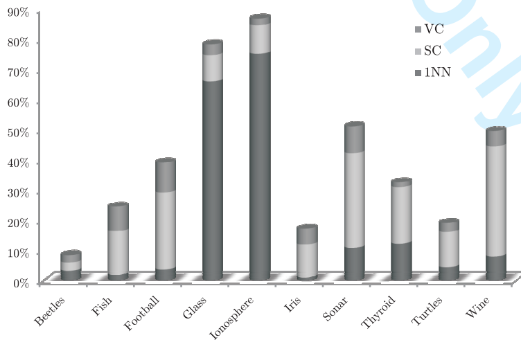
FIGURE 14. Cumulative percentage of wins for real datasets
