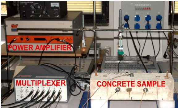
Fig. 2: NWMS test of reinforced concrete samples
