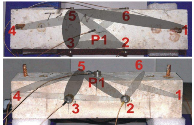
Fig. 4: NWMS pseudo-tomography imaging of damaged zones in reinforced concrete sample (corroded reinforcement separation).
