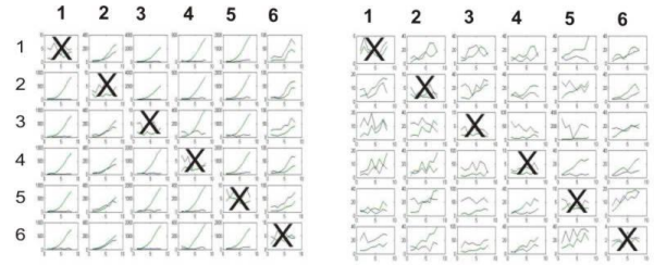
Fig. 3: Matrixes of 3rd harmonics (left) and frequency mixing products (right) for both intact (blue) and damaged (green) samples in dependence on growing f_{low} amplitude
