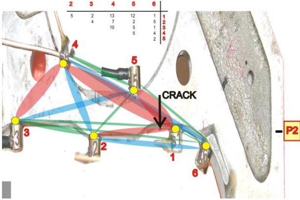
Fig. 5: NWMS pseudo-tomography imaging of the cracked zone in the ASB aircraft part subjected to fatigue loading.
