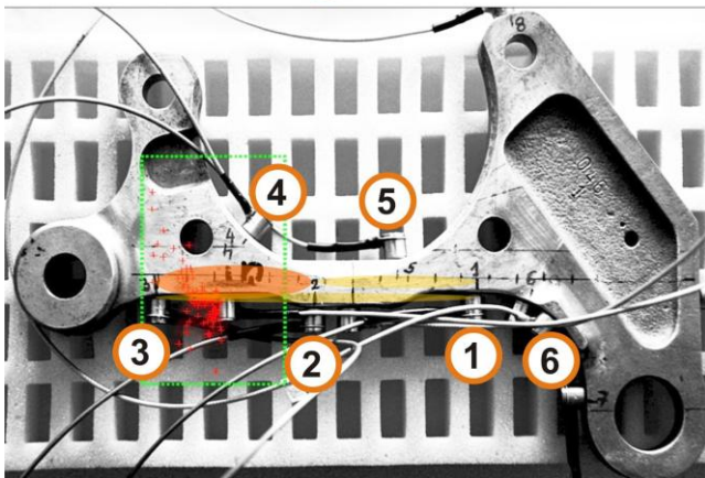
Fig. 6: ASB aircraft part with depicted zone of enhanced acoustic emission activity during the fatigue cycling. NLTRM pseudotomography imaging of potentially damaged zone with arising defect signaled already by acoustic emission.
