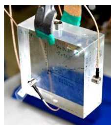
Fig. 1: Illustration of the pseudotomographic imaging of a cracked sample - schema and its practical realization on PMMA block with laser-induced crack
