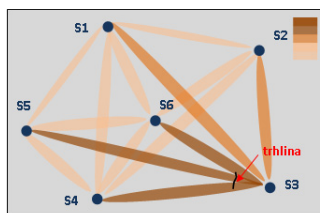
Fig. 1: Illustration of the pseudotomographic imaging of a cracked sample - schema and its practical realization on PMMA block with laser-induced crack
