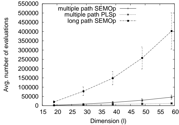
Fig. 6. Average value and standard deviation of the number of evaluations for PLS_p and SEMOp_p on biobjective multiple 2-path problems compared to the SEMOp_p on biobjective long 2-path.
