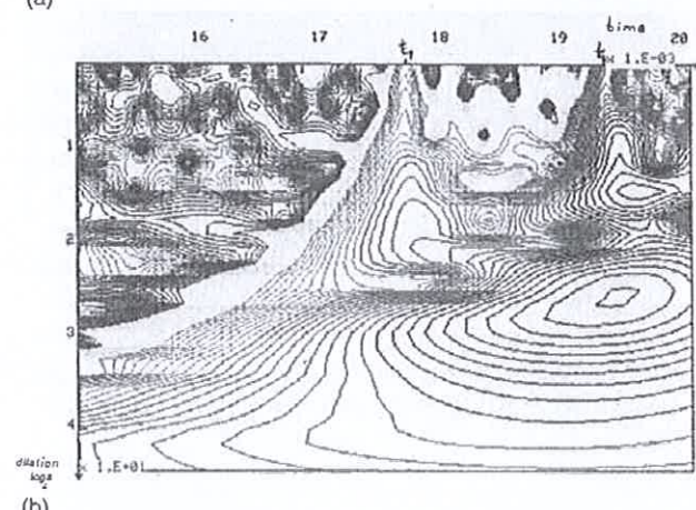
FIG. 10. Modulus of the wavelet transform of the total transmitted signal (experimental acoustic pressure field): (a) r=1 m, z=0.1 m, h=1 m; (b) r=1.5 m, z=0.1 m, h=1 m.
