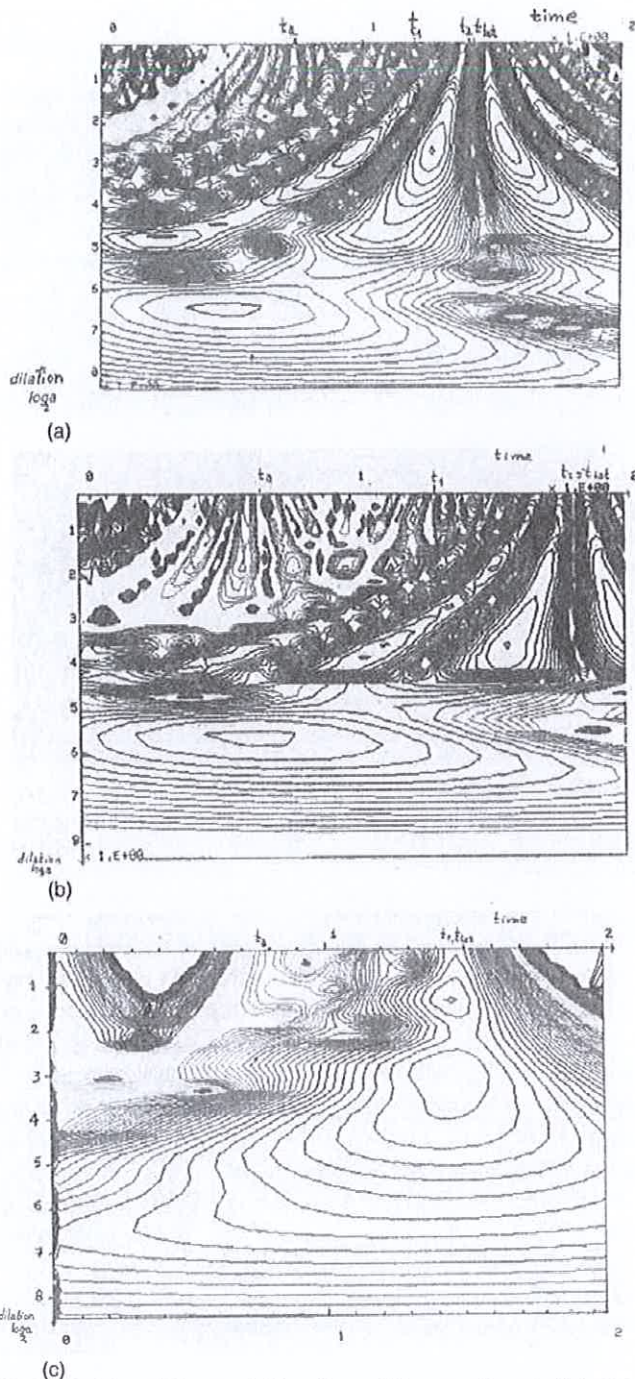
FIG. 5. Modulus of the wavelet transform of the acoustic potential associated to the "surface" contribution. The observation point is located at a radial distance larger than the sine of the critical angle and at the depth z/h=0.1 . (a) r/h=1 : the different arrival times are t_1=1.28 , t_2=1.414 , t_{lat}=1.436 , t_a=0.747 ; (b) r/h=1.5 , the different arrival times are t_1=1.314 , t_2=1.802 , t_{lat}=1.829 , t_a=0.634 ; (c) Modulus of the wavelet transform of the real part of the "surface" contribution at the observation point r/h=1 (radial distance) and z/h=0.1 (depth).
