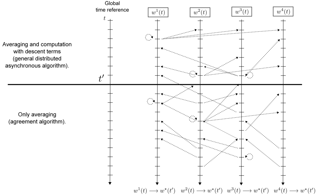
Figure 4: The agreement vector at time t' , w^*(t') corresponds to the common value asymptotically achieved by all processors if computations integrating descent terms have stopped after t' , i.e, s^j(t) = 0 for all t \geq t' .
