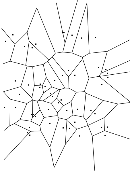
Figure 1: Voronoï tessellation of 50 points of \mathbb{R}^2 drawn uniformly in a square.
