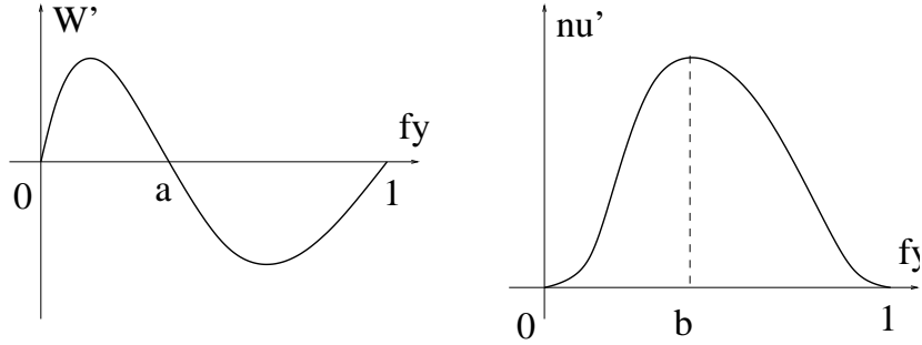
Figure 1: Derivatives of the double-well potential W and of the entropy coefficient \nu .
