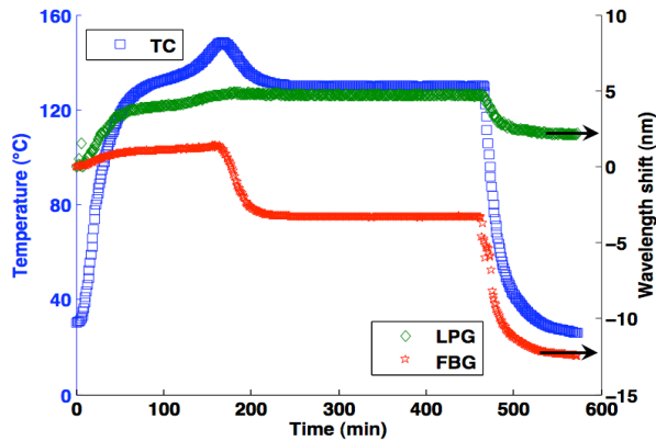
Fig. 4. Thermocouple temperature (left), FBG and LPG wavelength shifts (right) during epoxy resin curing
