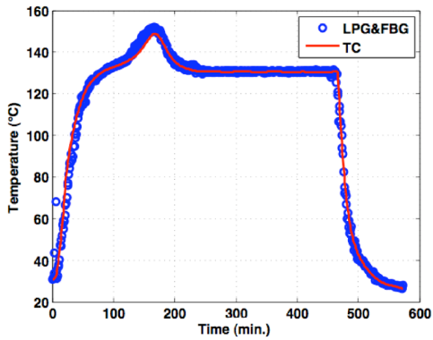
Fig. 5. Temperature measured with the superimposed LPG/FBG sensor during the curing process
