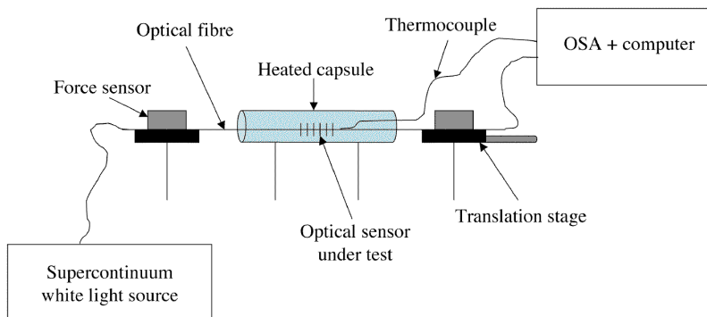
Fig. 1. Schematic diagram of the calibration bench
