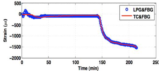
Fig. 9. Strain measured with the superimposed LPG/FBG sensor during the LRI process
