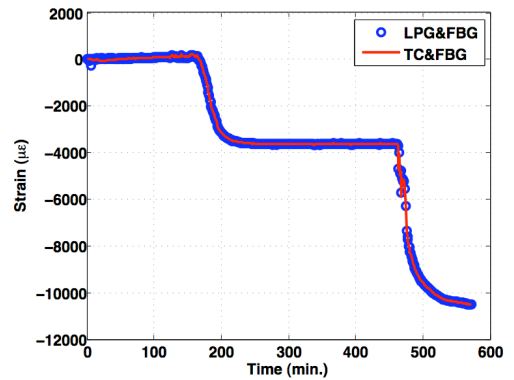
Fig. 6. Strain measured with the superimposed LPG/FBG sensor during the curing process
