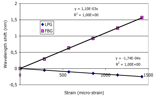
Fig. 3. LPG and FBG wavelengths shift in air as function of strain at 24°C.
