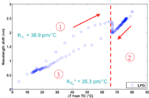
Fig. 10. LPG wavelength shift as function of temperature measured by thermocouple
