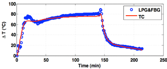
Fig. 8. Temperature measured with the superimposed LPG/FBG sensor during the LRI process
