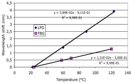
Fig. 2. LPG and FBG wavelengths shift in air as function of temperature with no strain.
