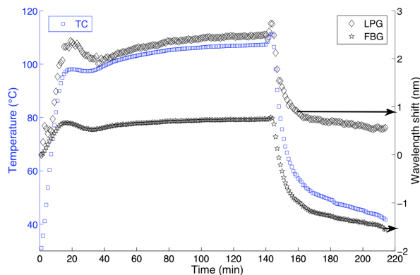
Fig. 7. Thermocouple temperature (left), FBG and LPG wavelength shifts (right) during the LRI process
