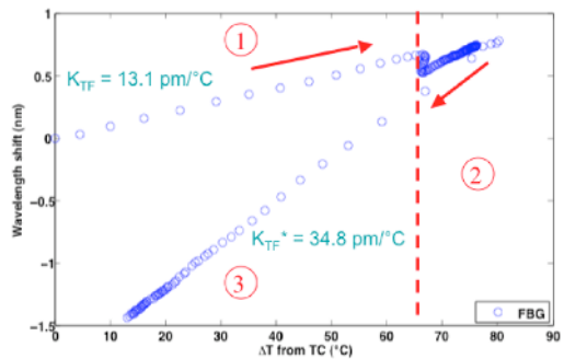
Fig. 11. FBG wavelength shift as function of temperature measured by thermocouple
