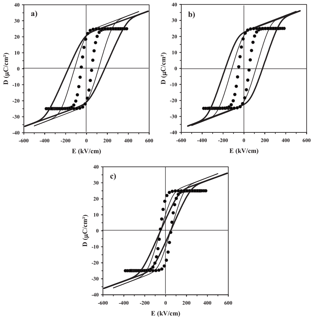
FIG. 6. Set of D - E hysteresis loops calculated from the model presented in Refs. 25 and 34. The loops before fatigue are in thin line, those after fatigue are in thick line. In dotted line is the inner P_f - E_f loop, i.e., the polarization loop due to the switching domains in the bulk ferroelectric layer from which were computed all the external D - E loops. The parameters used were the same as in Ref. 24 except those regarding the interface, chosen in such way to simulate three situations of fatigue: (a) fresh capacitors with C_i=4.7 nF and V_{bi}=\pm 3 V, fatigued capacitors with C_i=2.6 nF and V_{bi}=\pm 6 V, (b) fresh capacitors with C_i=4.7 nF and V_{bi}=\pm 3 V, fatigued capacitors with C_i=3.75 nF and V_{bi}=\pm 6 V, and (c) fresh capacitors with C_i=4.7 nF and V_{bi}=0 V, fatigued capacitors with C_i=2.6 nF and V_{bi}=0 V.
