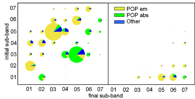
FIG. 5. (Color online) Intensity of scattering events between subbands. The size (area) of a given bubble represents the number of events. For each initial subband (y-axis) assign the final state after interaction—final subband (x-axis). The left part of the figure represents intrasegment scatterings; the right part, the scatterings to the right neighboring segment. Only scattering between first seven subband are plotted as scatterings to higher subbands are not visible in the scale of this figure.
