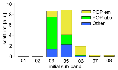
FIG. 6. (Color online) Scatterings responsible for filling upper lasing level. Scatterings starting from subbands higher than eighth, or from subbands belonging to neighboring segments are not visible in the scale of this figure.
