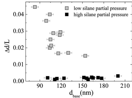
FIG. 6. Degree of tapering, defined as \Delta d/L=(d_{\text{base}}-d_{\text{top}})/L , as a function of the NW diameter for two different silane partial pressures. d_{\text{base}} and d_{\text{top}} are, respectively, the base and the top diameters of the SiNWs and L their length.
