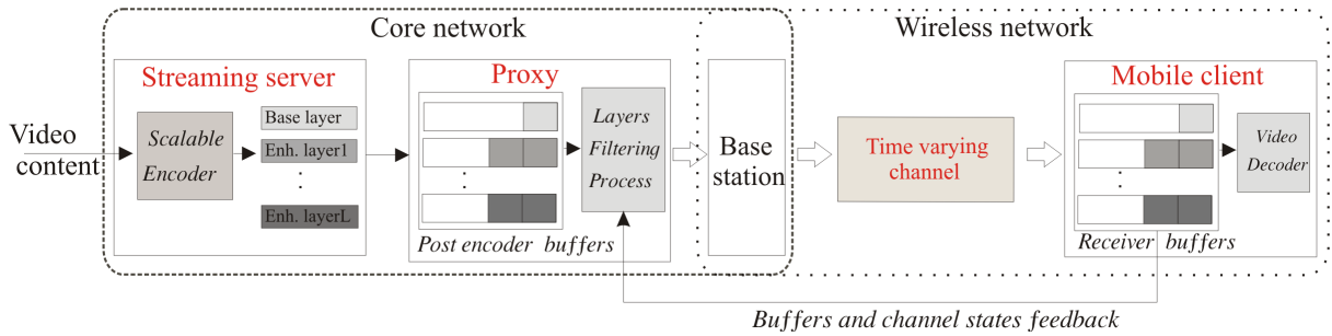
Figure 1: End-to-end video streaming scheme
