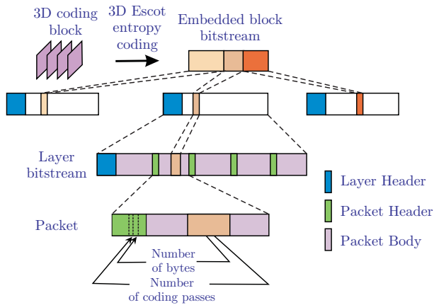
Figure 3: Packetisation Process
