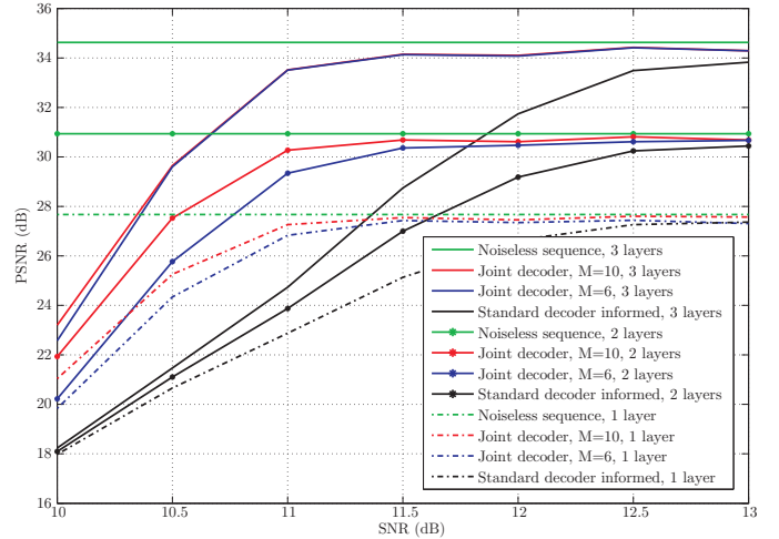
Figure 4: Average PSNR of the decoded sequence produced by an informed standard decoder and by the proposed JSCD as a function of the channel SNR when 1, 2, and 3 layers are decoded.
