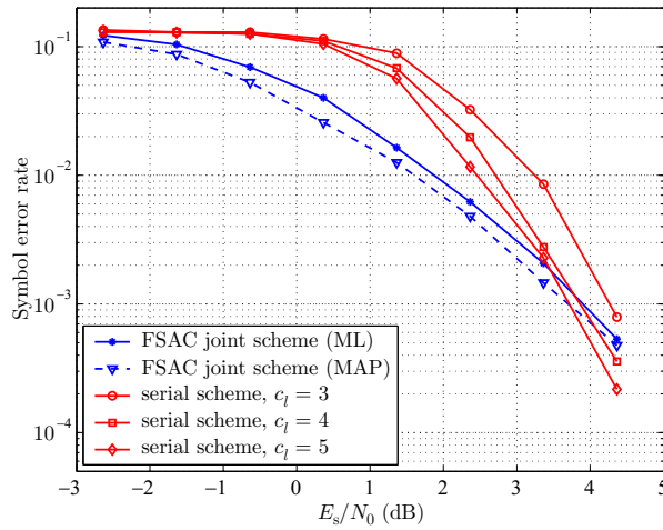
Fig. 6. Comparing the error correcting performance of the proposed joint scheme to a classical tandem scheme (AC + CC), using rate 7/8 punctured CC with c_l = 3 , c_l = 4 , and c_l = 5
