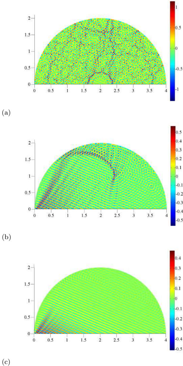
FIG. 9: Numerical simulations of a SAW inside an non-deformable half-spherical drop, f_0=20.375 MHz and d=2 nm. Colour levels stand for pressure. (a) Weak attenuation in the case of water. (b) Intermediate attenuation, 25 times larger than (a). (c) Strong attenuation, 100 times larger than (a).
