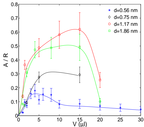
FIG. 7: Amplitude of the creeping-jumping oscillations of water droplets versus volume, for various acoustic displacements. The curves are guidelines for the eye.
