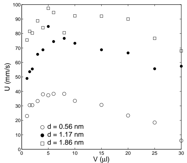
FIG. 4: (a) Drop velocity versus acoustic displacement d , for 3 different volumes (water). (b) Drop velocity versus volume, for 3 values of d .
