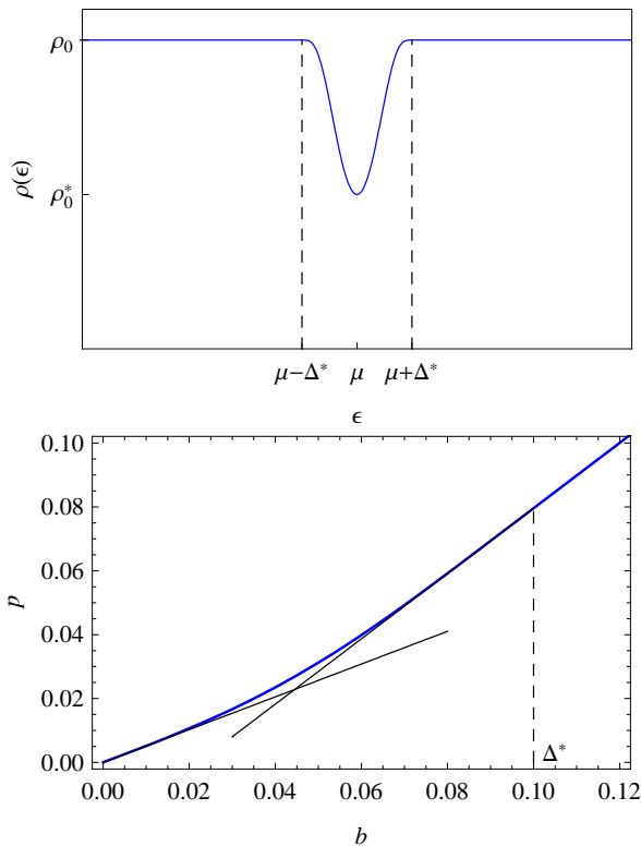
FIG. A2: Top: sketch of the density of state in a pseudogap model. A footprint of the molecular state appears as a dip of width \Delta^* and depth \rho_0 - \rho_0^* in the density of state. Bottom: Polarization p as a function of the magnetic field b , with \rho_0^* = 0.5\rho_0 and \Delta^* = 0.1\mu . At low imbalance, the Fermi levels of the two spin species lie inside the dip. This results in a depletion of spin excitations and a reduction of the spin susceptibility.
