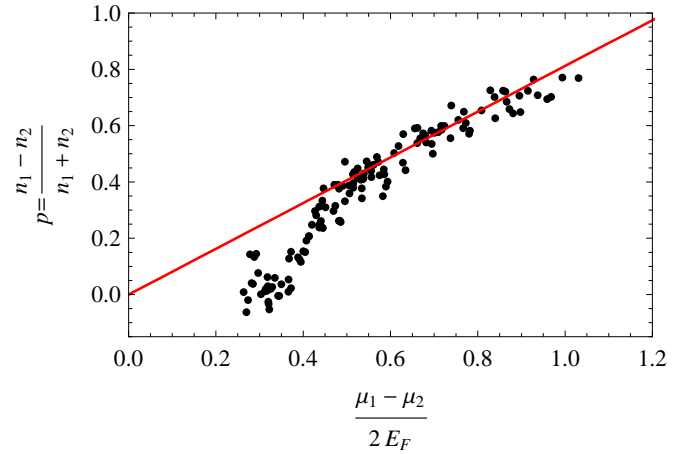
FIG. A3: Polarization p of the unitary Fermi gas as a function of the magnetic field \mu_1 - \mu_2 , normalized to the Fermi energy E_F = \hbar^2/2m(3\pi^2n)^{2/3} . The red line corresponds to the relation p = \frac{3}{2}\tilde{\chi}(\mu_1 - \mu_2)/2E_F , with \chi = 0.54 .
