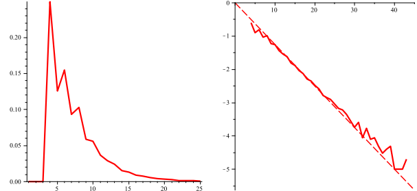
Figure 6: The distribution of costs of the Machin machine (4.15). Left : histogram. Right : decimal logarithms of the probabilities, compared to \log_{10}(10^{-k/8}) (dashed line).
