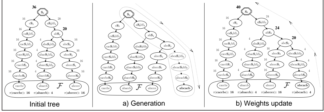
Figure 3: Prefix tree built from the subset \mathcal{F} = \{\text{cacbc}, \text{abaccb}, \text{abcccc}\} of Motzkin words of size 6, using weights \pi(a) = \pi(b) = 1 and \pi(c) = 2 . Generation (a) of a new word \text{abcacb} and update (b) of the contributions of \mathcal{F} to the immature words involved in the generation.
