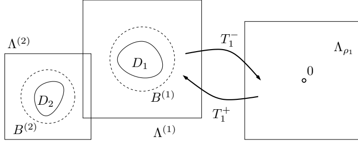
Figure 2: 2D-Sketch of a scatterer consisting of two parts D_1 and D_2 . The cylinders B^{(1)} = o_1 + B_{\rho_1/2} and B^{(2)} = o_2 + B_{\rho_2/2} are contained in the boxes \Lambda^{(1)} and \Lambda^{(2)} , respectively. The computational domain \Lambda_{\rho_1} is the reference domain for \Lambda^{(1)} and T_1^\pm transport functions between the two domains.
