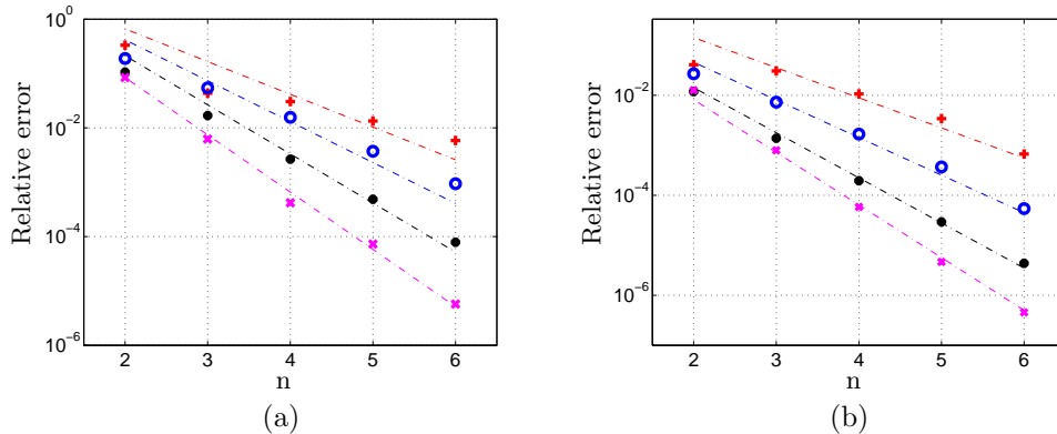
Figure 4: Relative L^2 -error of the projection/multipole method (64)(a) and the collocation/multipole method (64)(a) for waveguide medium scattering from two inclusions \mathbf{q} \in \mathbf{W}^s for s < \alpha + 3/2 and \alpha = 0, 1/2, 1, 3/2 . Pluses, circles, dots, and crosses correspond to \alpha = 0, 1/2, 1 , and 3/2 , respectively. The dotted lines correspond to convergence order 3/2 + \alpha . (a) Collocation method: relative error versus n , l = (2^n, 2^n, 2^n)^\top . (b) Projection method: relative error versus n , l = (2^n, 2^n, 2^n)^\top .
