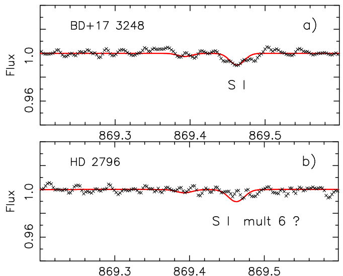
Fig. 1. Spectra of BD+17 3248 and HD 2796, showing the line at 869.46 nm in Mult. 6 of S I. We detect the line in BD+17 3248 ([Fe/H]=-2.1), but not in HD 2796 ([Fe/H]=-2.5). A synthetic spectrum (full line) corresponding to the equivalent width of 0.26 pm found by Israelian & Rebolo for this line has been superimposed on our spectrum of HD 2796.
