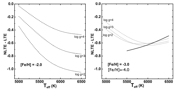
Fig. 3. NLTE correction for the 921.2nm sulphur line in metal-poor stars as a function of the temperature, the gravity and the metallicity for [\text{Fe}/\text{H}]=-2 , [\text{Fe}/\text{H}]=-3 (dashed lines) and [\text{Fe}/\text{H}]=-4 (solid line). This correction has been computed for [\text{S}/\text{H}]=[\text{Fe}/\text{H}] .
