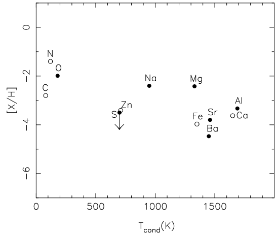
Fig. 7. [X/H] abundances in CS 22949-037 against the solar condensation temperatures (Lodders, 2003). There is no correlation between T_{\text{cond}} and the abundance of the elements, in particular S and Zn have a condensation temperature lower than Na and they are more deficient, at variance with the abundances in \lambda Boo stars. (The filled circles represent the abundances corrected or not sensitive to NLTE effects, the open symbols are abundances which could not be corrected for NLTE effects)
