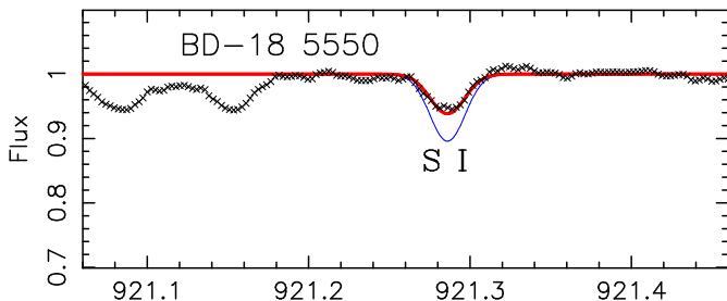
Fig. 5. Spectrum of BD-18 5550 in the region of Mult. 1 of S I. Only the main line can be measured in our spectrum, as the others are severely blended with telluric lines. The thick line shows the theoretical profile computed with our value of the S abundance (Table 3). The profile computed with the abundance adopted by Takeda & Takada-Hidai (2010) (thin line), is not compatible with the observed spectrum.
