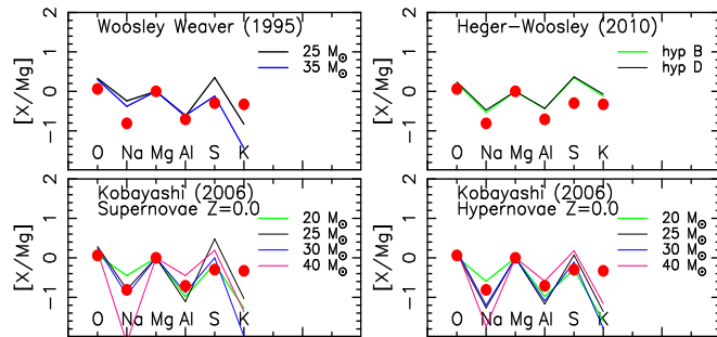
Fig. 8. Comparison of the most recent O, Na, Mg, Al, S, and K abundances in EMP stars to the predicted yields of metal-poor SNe and hypernovae. The solid lines represent the predictions of different models, and the dots the mean values of the observed abundances in the interval -3.0 < [Mg/H] < -2.0
