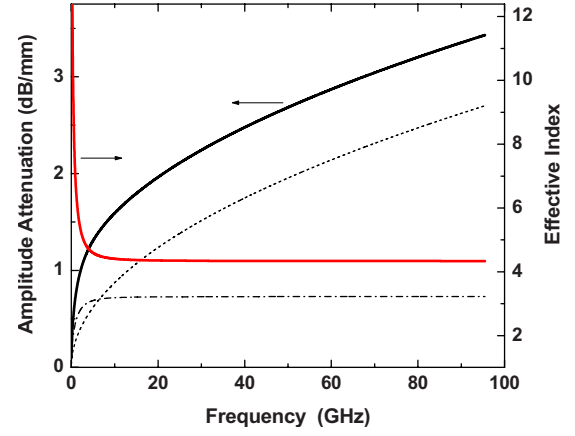
FIG. 3. (Color online) Microwave attenuation (black curve, left axis) and effective index (red curve, right axis) derived from the distributed parameters. As shown by the dashed lines the attenuation is given by the sum of two contributions: (i) a virtually frequency independent component due to the shunt conductance (dashed-dotted line) and (ii) a \sqrt{f} -dependent contribution stemming from the series resistance (dotted line).
