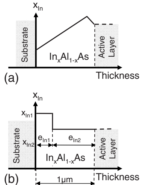
FIG. 1. Schematics of the variations in indium composition in metamorphic InAlAs buffers on InP(001): (a) graded ones and (b) two-step ones (this study).
