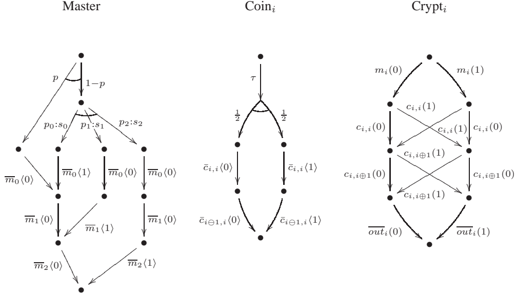
Fig. 3. Dining Cryptographers Automata
