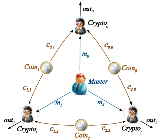
Fig. 1. Chaum's system for the Dining Cryptographers ([9])
