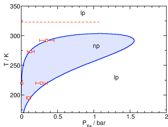
Figure 2. Temperature-xenon pressure phase diagram of MIL-53(AI). Solid line: osmotic thermodynamic model. Open symbols: experimental transition steps in the isotherms. The dashed line corresponds to the experimental temperature (323 K) for which no transition took place.
