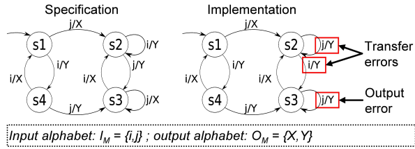
Figure 4: Example of transfer and output errors in a Mealy machine
