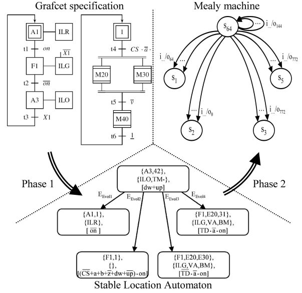
Figure 5: Method overview
