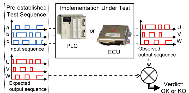
Figure 1: Conformance test principle
