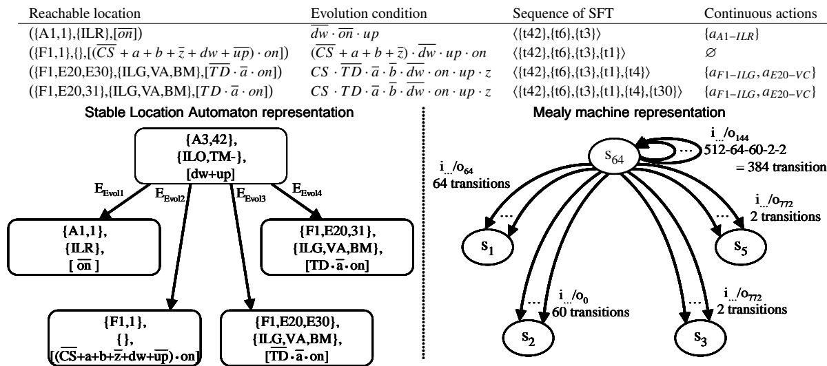
Figure 6: Representation of evolutions from location ((A3,42),\{ILR\},[dw + up]) using the SLA and the Mealy machine representations for the example given figure 3
