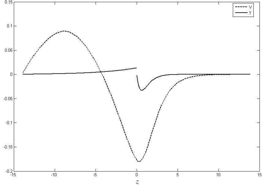
Figure 1: Velocity (dashed line) and temperature (solid line) distributions without vibration for R = 20 , k = 0.7195 , Z = 8 , P = 0.5 .
