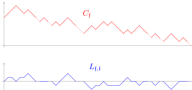
Figure 4: The contour pair of the well-labeled forest appearing in Figure 3. The paths are dashed on the intervals corresponding to floor edges.
