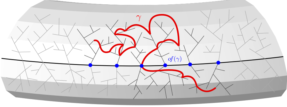
Figure 7: The set overflowed by the path \gamma is the set of (blue) large dots.
