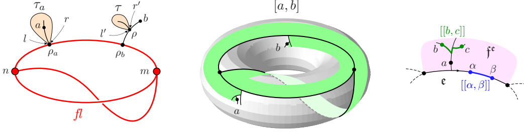
Figure 6: Left. On this picture, we can see the floor fl , the two nodes n and m , an example of tree \tau_a , and an example of tree \tau on the left of [[\rho_b, b]] rooted at \rho . Middle. The set [a, b] . Right. On this picture, a is an ancestor of b and c , and we can see the sets [[b, c]] , [[\alpha, \beta]] , and f^\epsilon .
