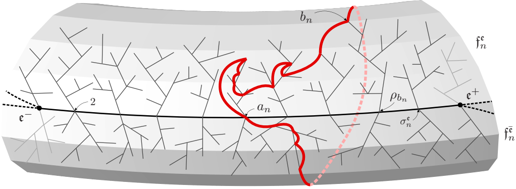
Figure 11: A non-contractible loop intersecting fl_n at a_n and “jumping” from \mathfrak{f}_n^e to \mathfrak{f}_n^{\bar{e}} at b_n .
