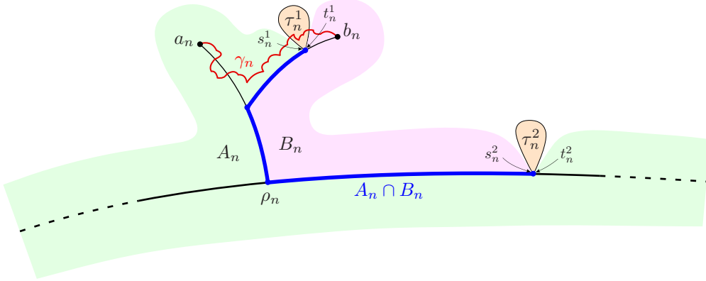
Figure 10: The path \gamma_n passing through the subtree \tau_n^1 .
