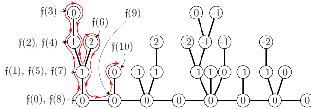
Figure 3: The facial sequence of a well-labeled forest from \mathfrak{F}_7^{20} .
