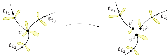
Figure 13: Slicing an intertwined node v .
