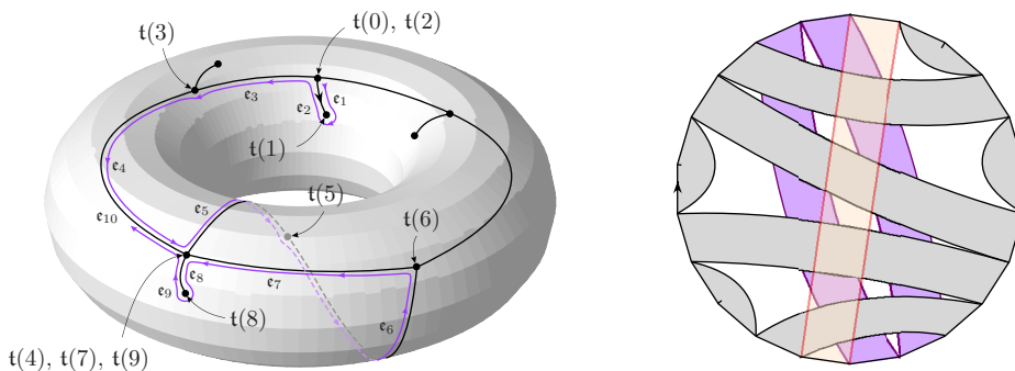
Figure 1: Left. The facial order and facial sequence of a g -tree. Right. Its representation as a polygon whose edges are pairwise identified.
