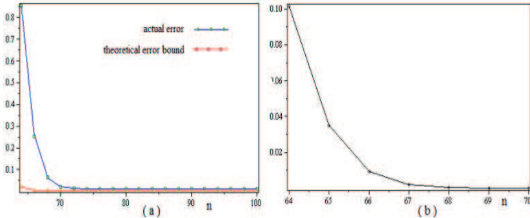
Figure 2: (a) Graphs of the theoretical and the actual error bound for example 2. (b) Graph of the decay of \lambda_n(c) .
