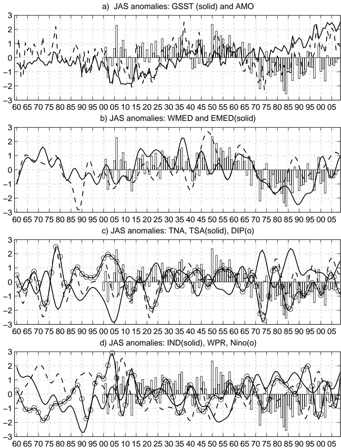
Figure 2. Time evolution of the July-September standardized time series of Sahel rainfall (bars) on the period 1900-2008 and of a few selected low frequency SST anomaly indices (superimposed curves) over the period 1860-2009).
