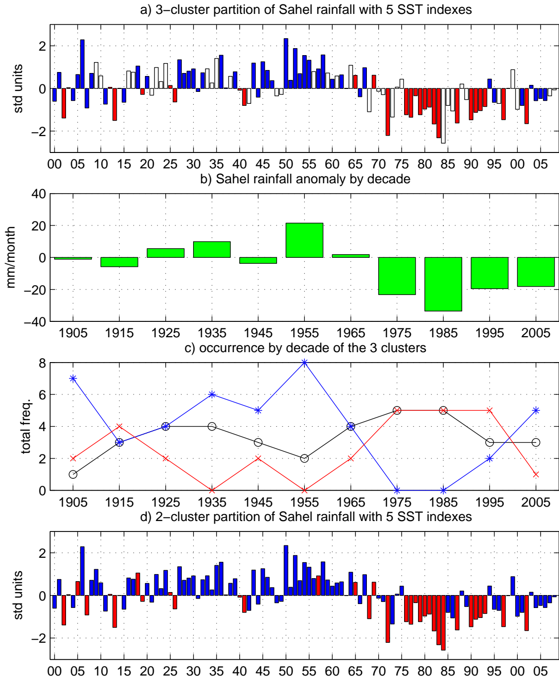
Figure 4. Time projections of the Kmeans results displayed in Table 3 onto the standardized Sahel rainfall series at an interannual timestep (a,d) and co-variation with Sahel rainfall in mm/month over 10-year sub-periods (b,c) between 1900 and 2008: AP (white), MAI (blue) and MIP (red).
