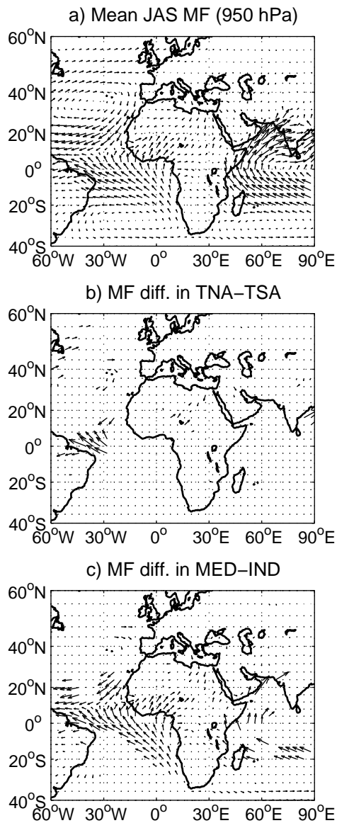
Figure 7. July-September moisture flux at 950 hPa over the period 1920-2008. (a) mean values; (b) significant differences between the northern and southern tropical Atlantic basins; (c) significant differences between the eastern Mediterranean basin and the Indian Ocean. The statistical significance has been estimated on the zonal and meridional components through a Student t-test contrasting the 20 highest and the 20 lowest seasonal differences versus all the remainders.
