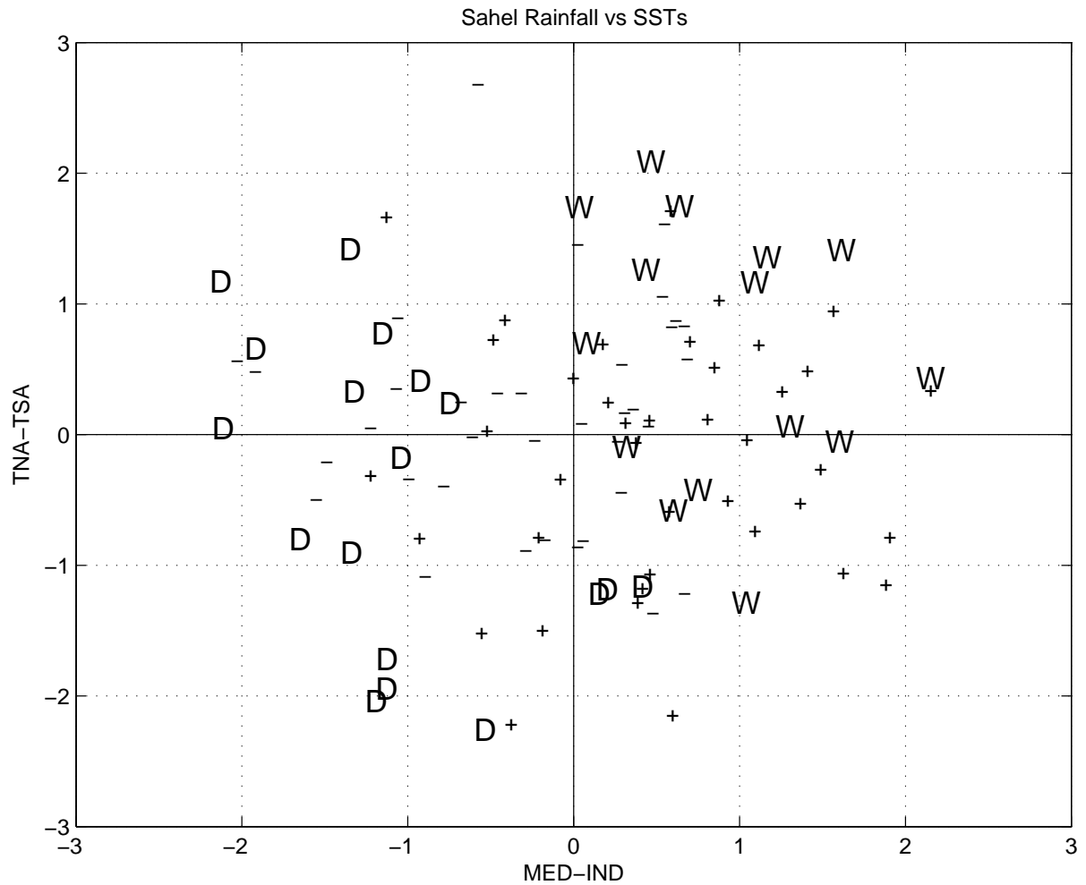
Figure 5. Scatter-plot of summertime (JAS) Sahelian rainfall as a function of the differences computed between the MED and IND (x-axis) and TNA and TSA (y-axis) standardized time series. 'W' ('D') denote the wettest (driest) rainfall anomalies, i.e., those exceeding 1 sd in absolute value, while '+' and '-' refer to other positive (negative) anomalies. Period. 1900-2008.
