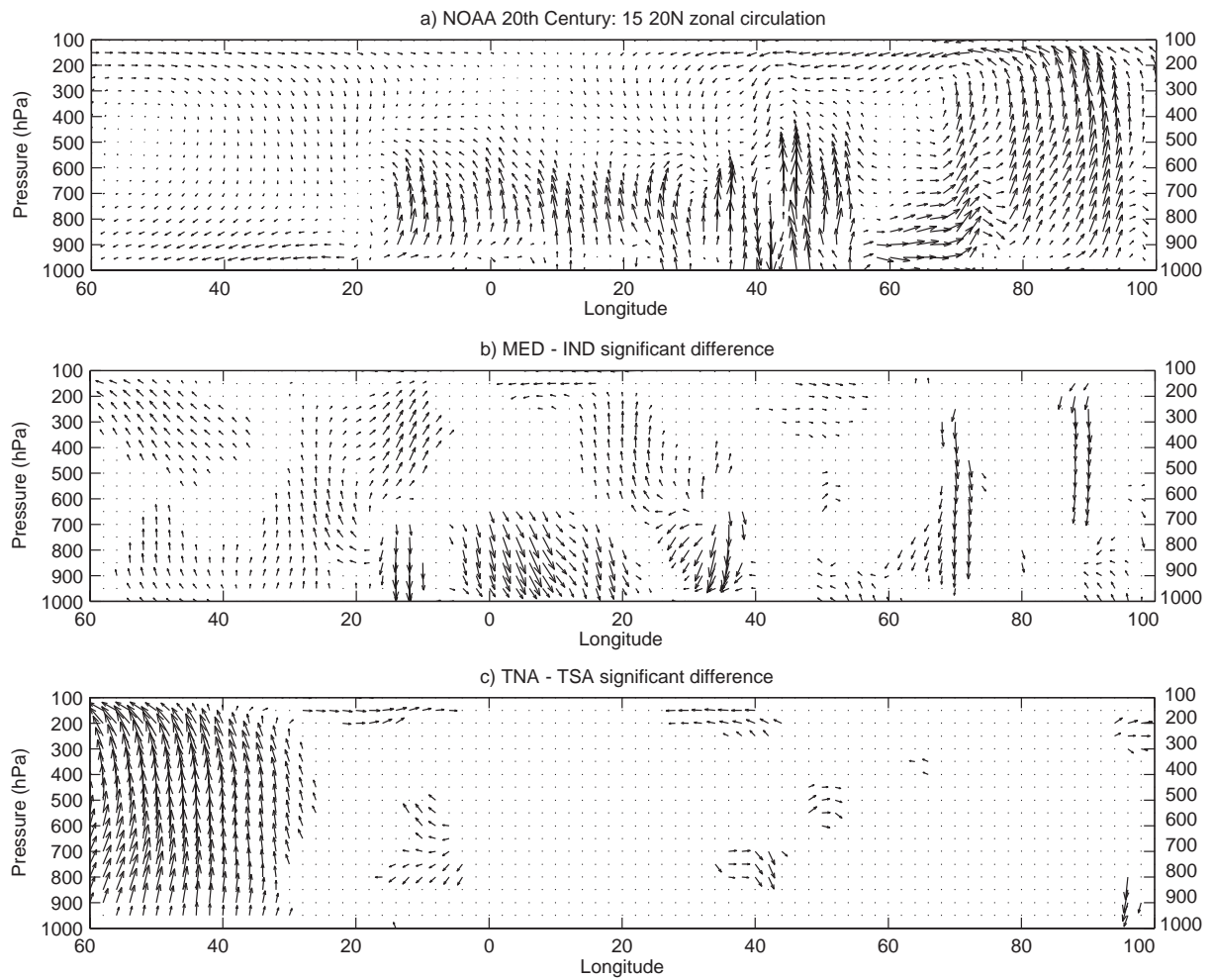
Figure 9. As figure 8 but for the July-September atmospheric circulation along a zonal-vertical plane averaged between 15°N and 20°N.
