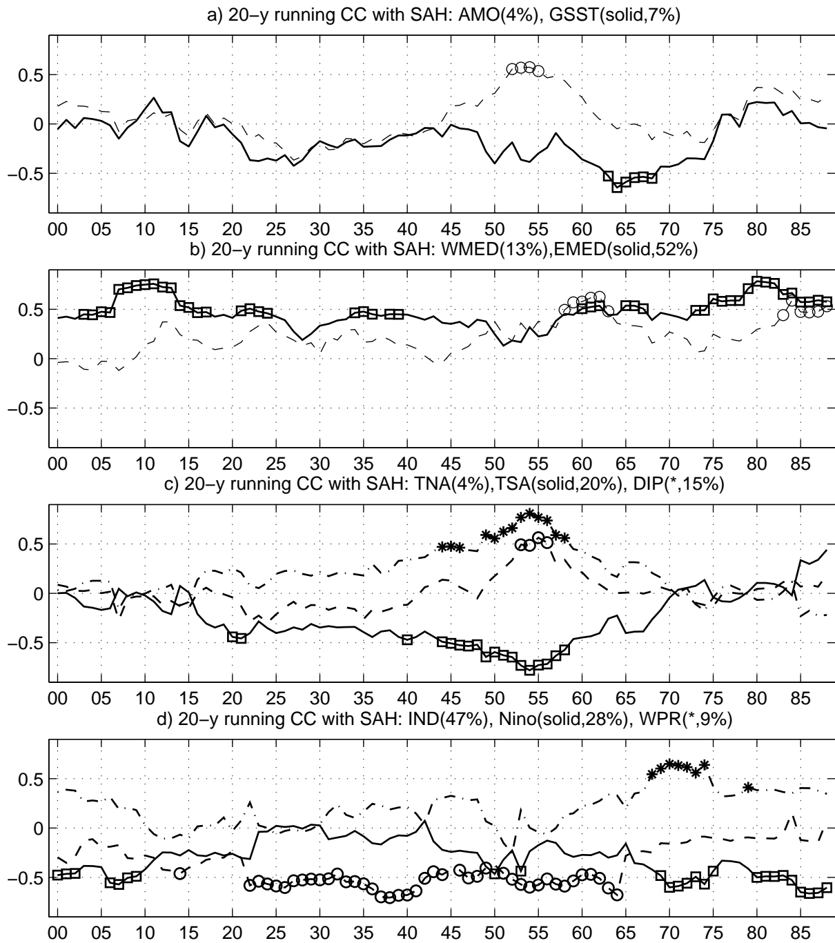
Figure 3. Correlation coefficients computed on 20-year running windows between the Sahel rainfall index and the SST indexes displayed in figure 2.
