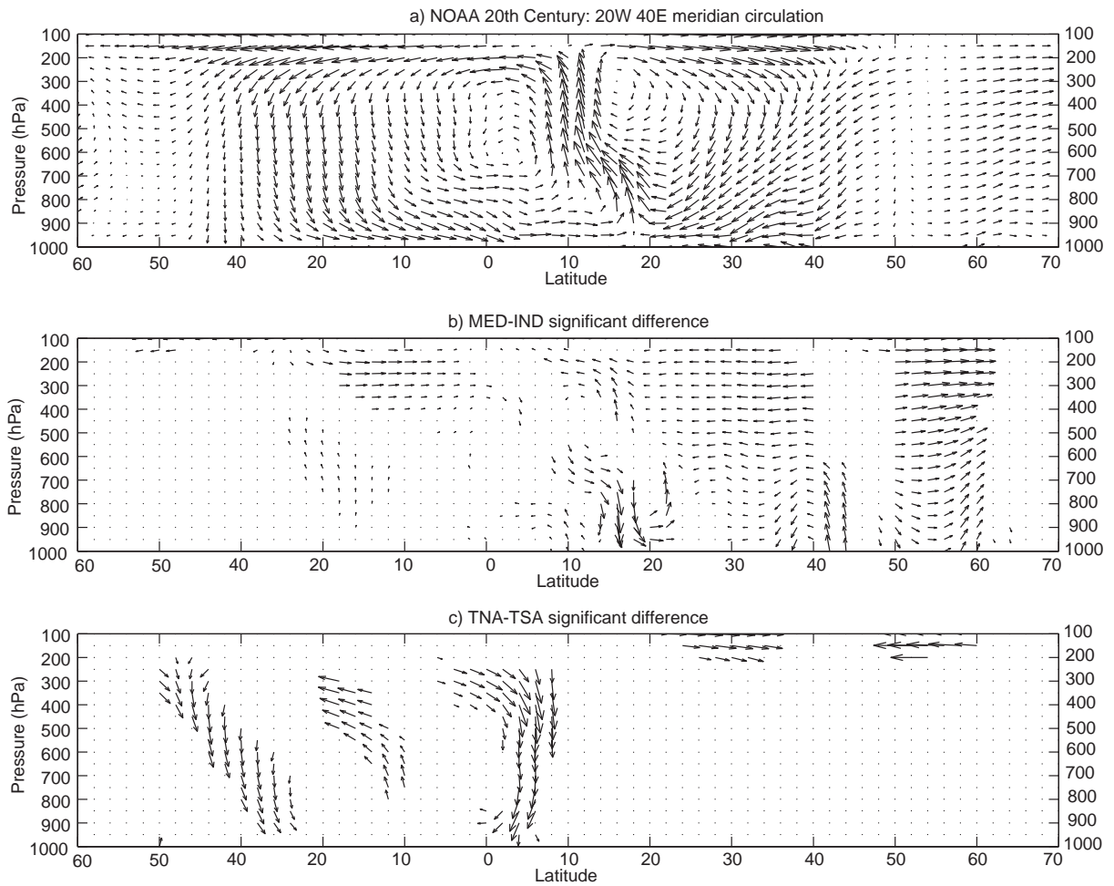
Figure 8. July-September atmospheric circulation (divergent wind, -\omega ) along a meridional-vertical plane averaged between 20^{\circ}\text{W} and 40^{\circ}\text{E} over the period 1920-2008. (a) Mean values; (b) MED-IND composite relative to SST differences between the eastern Mediterranean basin and the Indian Ocean (c) TNA-TSA composite relative to SST differences between the northern and southern tropical Atlantic basins. In panels (b,c) only the significant values are displayed. The statistical significance has been estimated on the vertical and meridional components through a Student t-test contrasting the 20 highest and the 20 lowest seasonal differences versus all the remainders.
