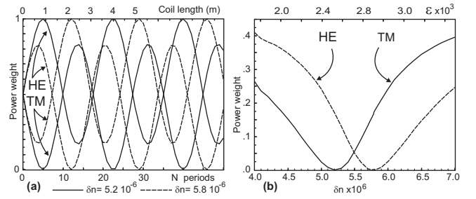
Fig. 2. Intermodal coupling: (a) normalized power of HE_{21}^{ev} and TM_{01} vs. coiling length for R = 20 mm, \Lambda = 177.6 mm and 2 values of the birefringence \delta n , (b) minimum of |(HE_{21}^{ev})|^2 and |(TM_{01})|^2 vs. \delta n
