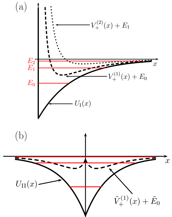
FIG. 3: (color online). (a) Potential U_I(x) with 3 bound states (red lines) and its first two supersymmetric partners V_+^{(1)}(x) + E_0 and V_+^{(2)}(x) + E_1 ( a = 11.75 ). (b) Potential U_{II}(x) with 3 bound states (red lines) and its first supersymmetric partner \tilde{V}_+^{(1)}(x) + \tilde{E}_0 that has a double well shape ( a = 4.5 ).
