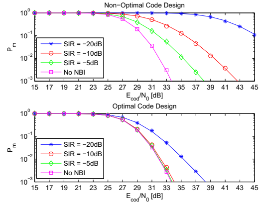
Fig. 3. Miss Probability ( P_m ) against E_{cod}/N_0 . Setup with \hat{\mu}_c = 0 and \hat{\mu}_w = 2 . Markers: Monte Carlo simulation; solid lines: analytical model.
