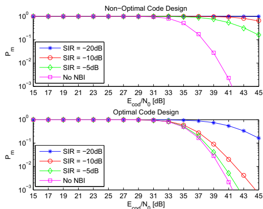
Fig. 5. Miss Probability ( P_m ) against E_{cod}/N_0 . Setup with \hat{\mu}_c = 0 and \hat{\mu}_w = 6 . Markers: Monte Carlo simulation; solid lines: analytical model.
