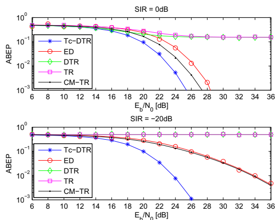
Fig. 1. ABEP against the Bit-Energy-to-Noise-Spectral-Density-Ratio ( E_b/N_0 ) and the Signal-to-Interference-Ratio (SIR). Legend: TR = Transmitted-Reference [16], DTR = Differential Transmitted-Reference [16], ED = Energy Detector [18], CM-TR = Coded-Multiplexed Transmitted-Reference [12], T c -DTR = Chip-Time Differential Transmitted-Reference [10]. A setup similar to [13, Fig. 1 and Fig. 2] is considered.
