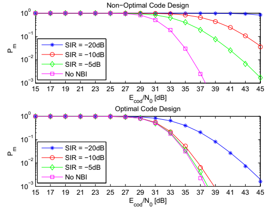
Fig. 4. Miss Probability ( P_m ) against E_{cod}/N_0 . Setup with \hat{\mu}_c = 0 and \hat{\mu}_w = 4 . Markers: Monte Carlo simulation; solid lines: analytical model.
