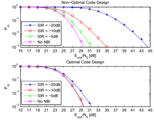
Fig. 2. Miss Probability ( P_m ) against E_{cod}/N_0 . Setup with \hat{\mu}_c = 0 and \hat{\mu}_w = 0 . Markers: Monte Carlo simulation; solid lines: analytical model.
