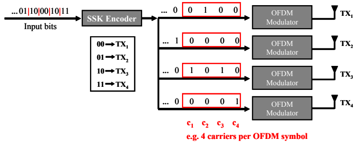
Fig. 1. Illustration of SSK in combination with OFDM.
