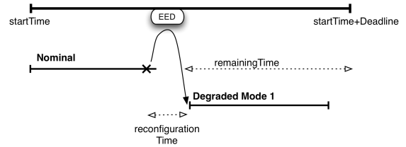
Figure 6. EED-based reconfiguration
