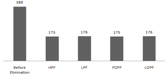
Figure 6. Average number of initial preemptions after preemption elimination
