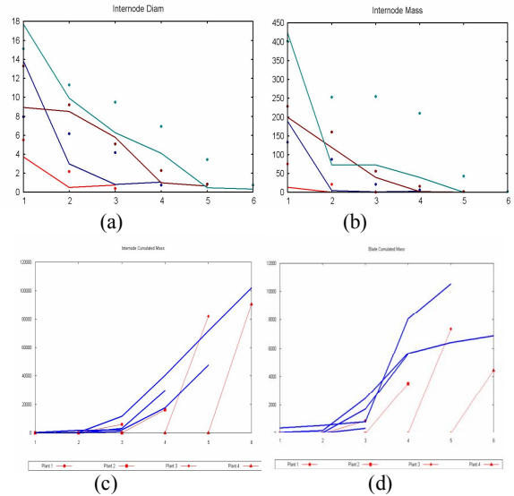
Figure 4. Multi-fitting results
