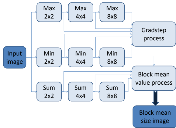
Fig. 9. Quad-Tree design
