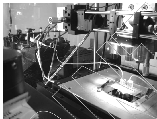
Figure 3: Picture of our microfluidic cell. The microscope coverslip is cleaned and chemically prepared and then taped to a microscope slide with small holes and PDMS blocks through which the reactants are injected for all the following steps of the surface chemistry and of the protein synthesis experiment.
