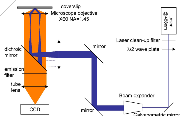
Figure 2: Schematics of our optical setup.
