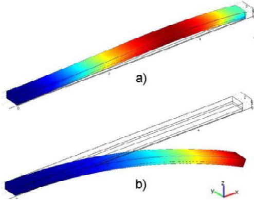
Fig. 7. FEM evaluation of: (a) blocking force mode and (b) free tip displacement mode of a 5.0x0.3x0.14 mm 3 PZT on Cu actuator submitted to 80 V in the polrization direction (-8.0 kV/cm). Deformed shapes are magnified around 50 times.
