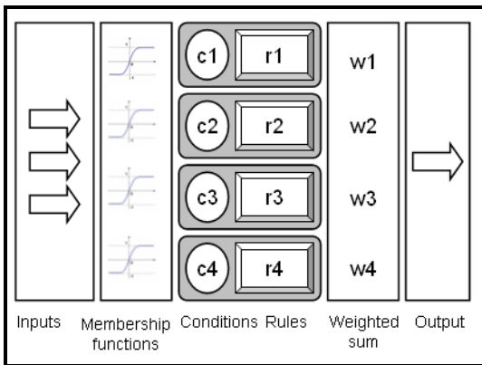
Fig. 2: The exTS with Condition-Rule modules.
