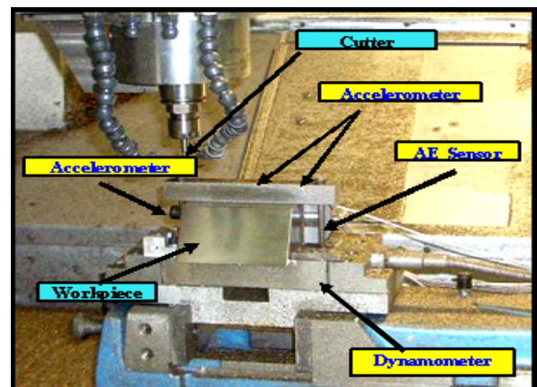
Fig. 3: The experimental set-up in a high speed milling machine
