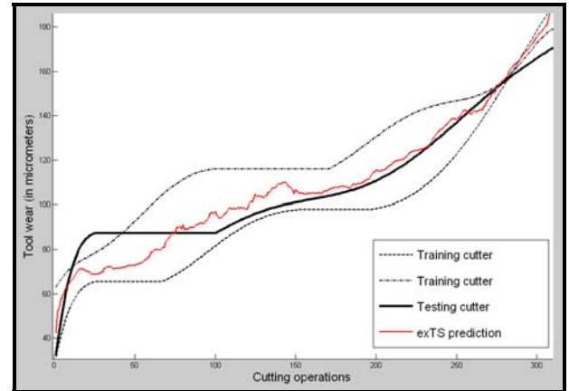
Fig. 9: Reliability performance on an unknown cutter.
