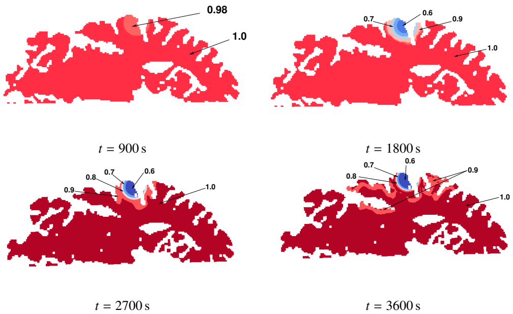
Figure 12: 3D simulation; cut by two perpendicular planes of the rADCw field at time t = 3600 s
