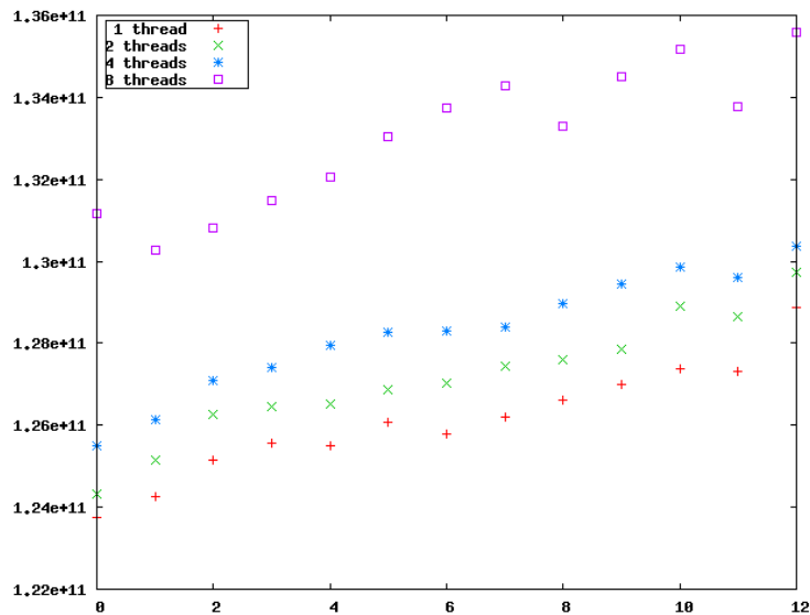
Figure 7: Performances of the multithreaded reaction solver along 12 time steps. Abscissa: time step. Ordinate: computing time in CPU clock ticks.
