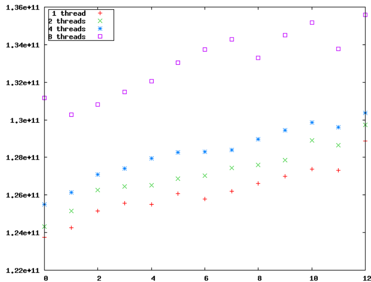
Figure 7: Performances of the multithreaded reaction solver along 12 time steps. Abscissa: time step. Ordinate: computing time in CPU clock ticks.
