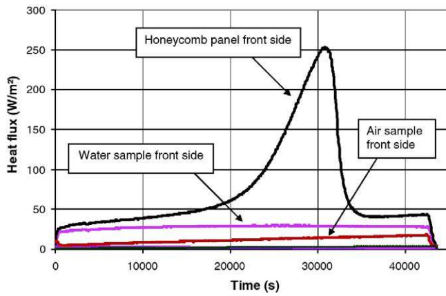
Fig. 8. Heat fluxes measured at the front sides of the three samples (PCM, water, air) during sample heating. Fluxes measured at the back sides are nearly zero.
