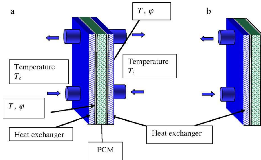
Fig. 3. Sketch of the experimental set-up: (a) both sides with imposed temperatures and (b) one side with an imposed temperature.
