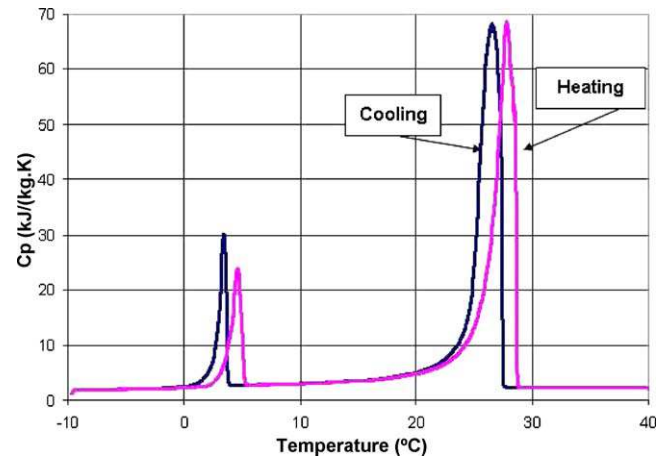
Fig. 1. Stored heat ( \sim C_p ) as a function of temperature measured by Differential Scanning Calorimetry (scanning rate, 0.05 K/min).
