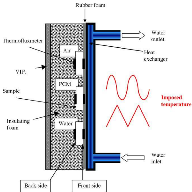
Fig. 5. Schematic of the test section with three samples and with temperature and flux sensors.
