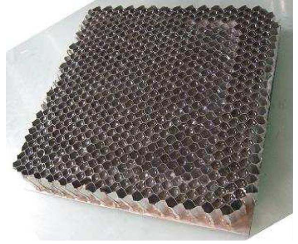
Fig. 2. Honeycomb panel sample filled with paraffin, before to stick the upper aluminium skin.
