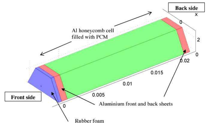
Fig. 10. Structure for the finite element modelling. Half of an aluminium hexagonal cell filled with PCM is represented with aluminium sheets of both sides. Rubber foam is placed on the front side.
