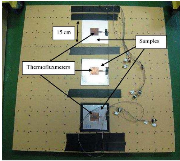
Fig. 4. The wall placed in the test loop. Three samples from up to down: empty (air), filled with PCM, filled with water.
