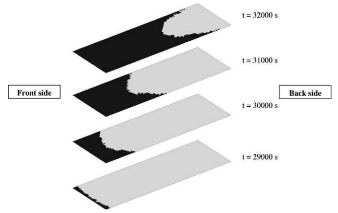
Fig. 11. Melting front propagation within the PCM in the symmetry plane of a honeycomb, for the time range [29,000;32,000 s]. In black, the liquid zone.
