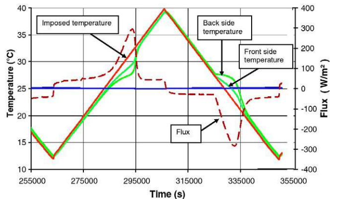
Fig. 7. Temperature (full lines) and flux (dotted line) variations of the PCM-filled honeycomb sample.
