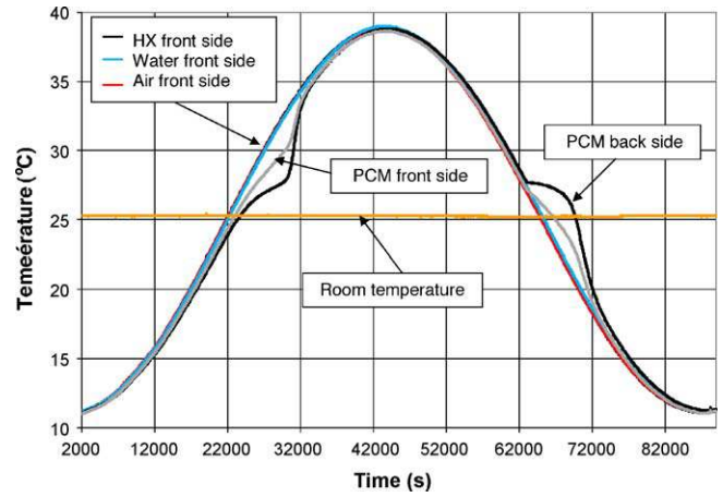
Fig. 9. Temperature variation for sinusoidal cycle. Pure sine curves are for imposed temperature, and front side temperatures of water and air samples.
