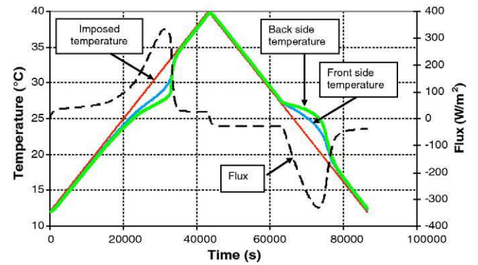
Fig. 12. Numerical prediction for temperature (full lines) and flux (dotted line) variations of the PCM-filled honeycomb sample.
