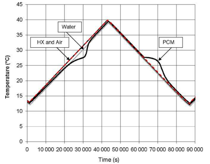
Fig. 6. Temperature variations on the back side of the empty sample (air – dotted line), the sample filled with water (water) and the honeycomb sample filled with PCM (PCM). Temperature of the heat exchanger (HX) is given for comparison.
