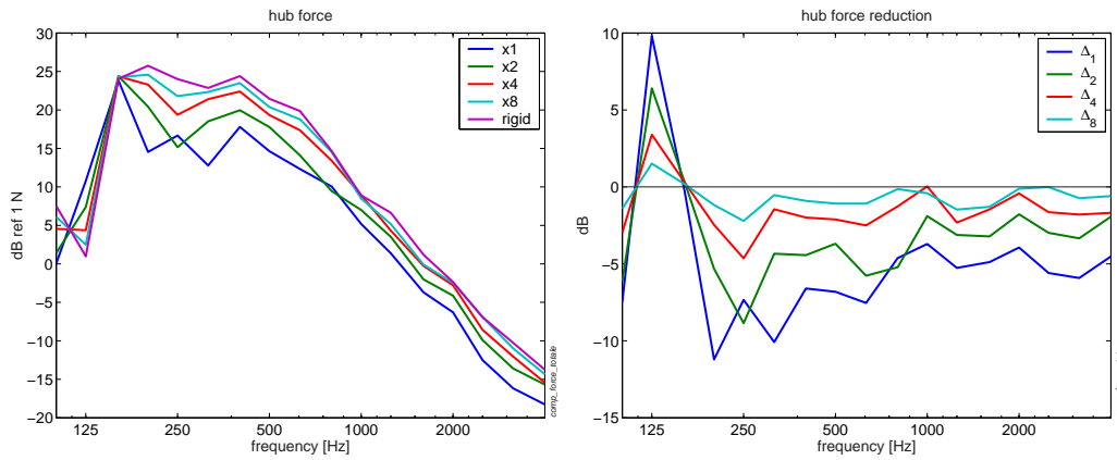
Figure 4.2: Hub force during the rolling process- left: spectrum levels- right: differences w.r.t. the rigid road case
