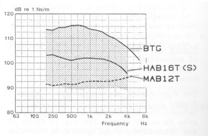
Figure 2.1: Mechanical impedance of road surfaces. Surfaces with high impedance in the high frequency domain [1]
