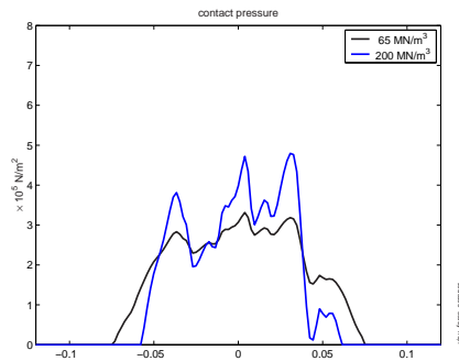
Figure 4.12: Instantaneous contact pressure for s_g = 65\text{MN/m}^3 and s_g = 200\text{MN/m}^3
