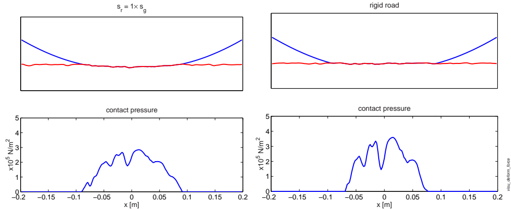
Figure 4.3: Tire and road profiles (upper) and contact pressure (lower) for a soft (left) and a stiff (right) pavement
