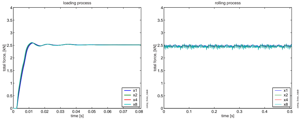
Figure 4.1: Global contact force. Left: loading process- Right: rolling process
