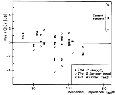
Figure 2.2: The residuals as a function of the mechanical impedance level (dB ref 1\tilde{N}s/m ) at 2000 Hz [3]
