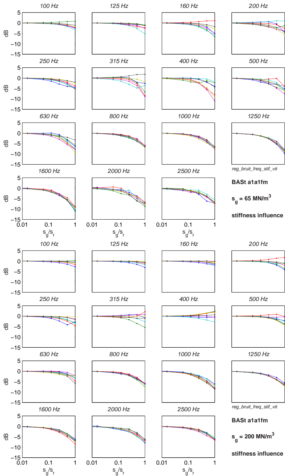
Figure 4.7: \Delta L_W = L_W(v, \mathbf{s}_r, f) - L_W(v, \infty, f) as function of s_g/s_r . The noise levels tend to decrease as the road becomes 'softer'
