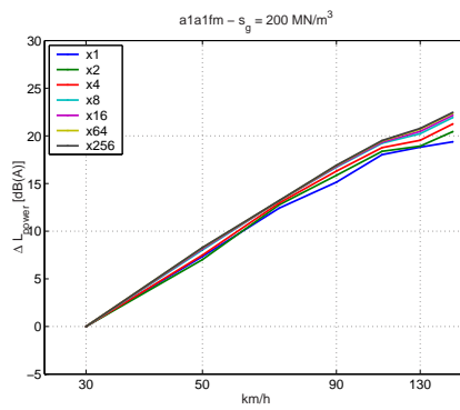
Figure 4.9: L_W(v, s_r, f) - L_W(30, s_r, f)
