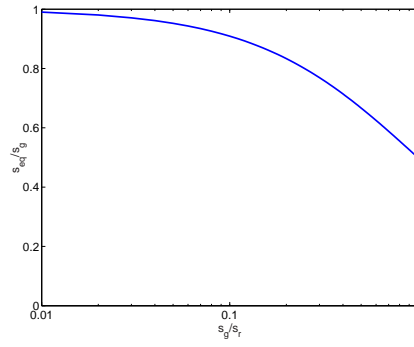
Figure 4.8: evolution of s_{eq}/s_g as function of s_g/s_r
