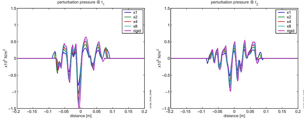
Figure 4.5: contact pressure : perturbation part at two instants
