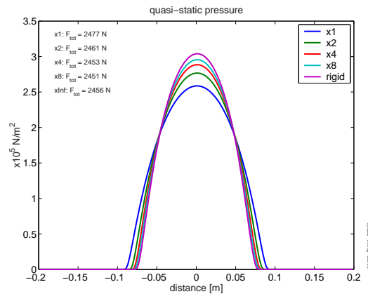
Figure 4.4: contact pressure : quasi-static part
