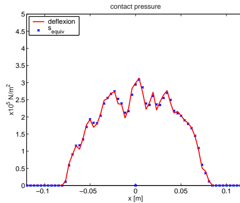
Figure 3.1: Contact pressure obtained by two methods § 3
