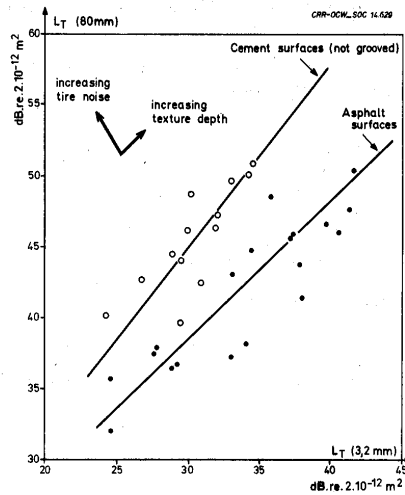
Figure 2.4: Comparison between asphalt and cement concrete surfaces based on their texture levels at the critical wavelengths with respect to tire/road noise [4]
