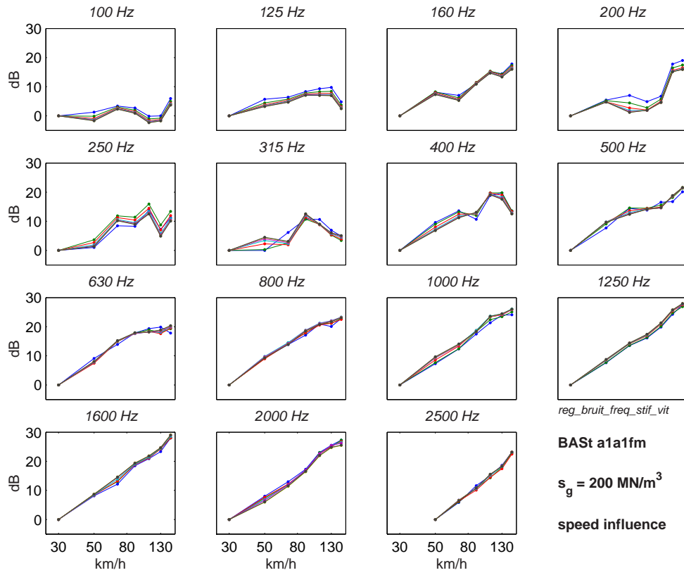
Figure 4.11: L_W(V, s - r, f) - L_W(30, s_r, f)
