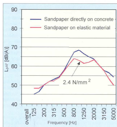
Figure 2.5: Effect of inserting a soft rubber layer between a sandpaper sheet and a cement concrete surface ( [6] cited in [7])
