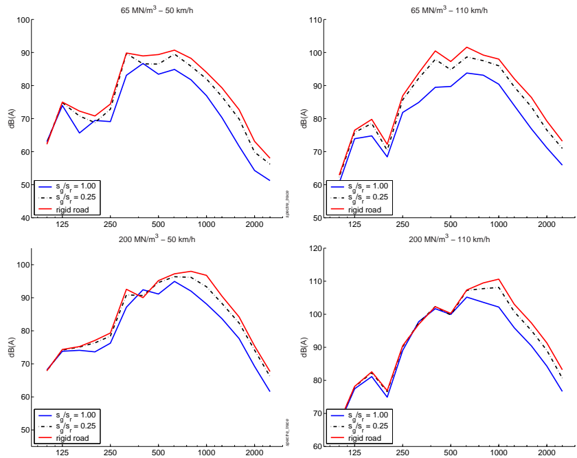
Figure 4.10: Power noise spectrum and road stiffness - left @ 50 km/h - right : @ 110 km/h
