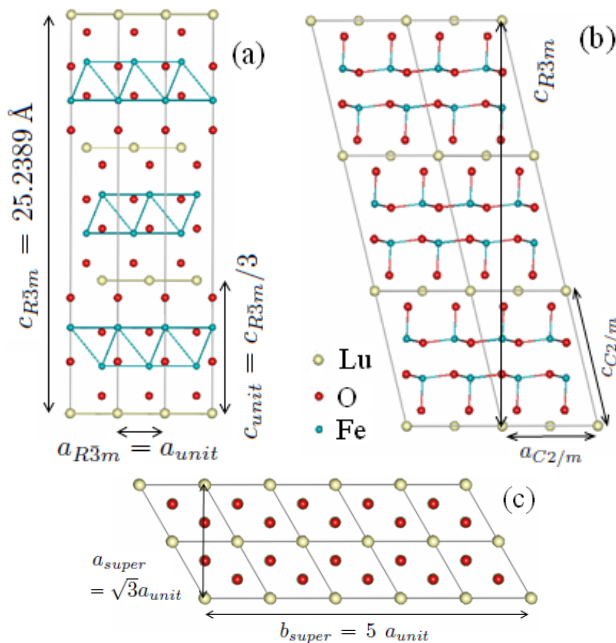
FIG. 1. a) (color online) Rhombohedral crystal structure of LuFe 2 O 4 . b) Equivalent monoclinic unit-cell of LuFe 2 O 4 C2/m with a_{C2/m} = 5.957 \text{ \AA} [ = a_{R3m}\sqrt{3} ], b_{C2/m} = 3.436 \text{ \AA} [ = a_{R3m} ] and c_{C2/m} = 8.641 \text{ \AA} [ \approx c_{R3m}/3 ] with \beta_{C2/m} = 103.2^\circ . c) Orthorhombic high-pressure modulated supercell: a_{super} \approx \sqrt{3}a_{unit} , b_{super} \approx 5a_{unit} and c_{super} \approx 8c_{unit} .
