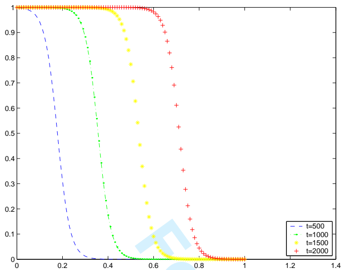
Figure 3. Asymptotic solutions for \epsilon = 0.02 and different values of t .
