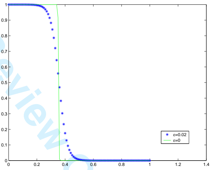
Figure 5. Asymptotic solutions for t = 1000 and different values of \epsilon
