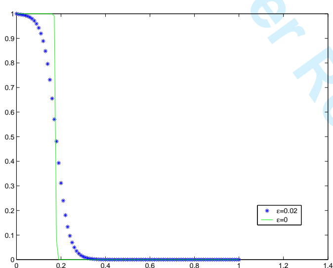
Figure 4. Asymptotic solutions for t = 500 and different values of \epsilon
